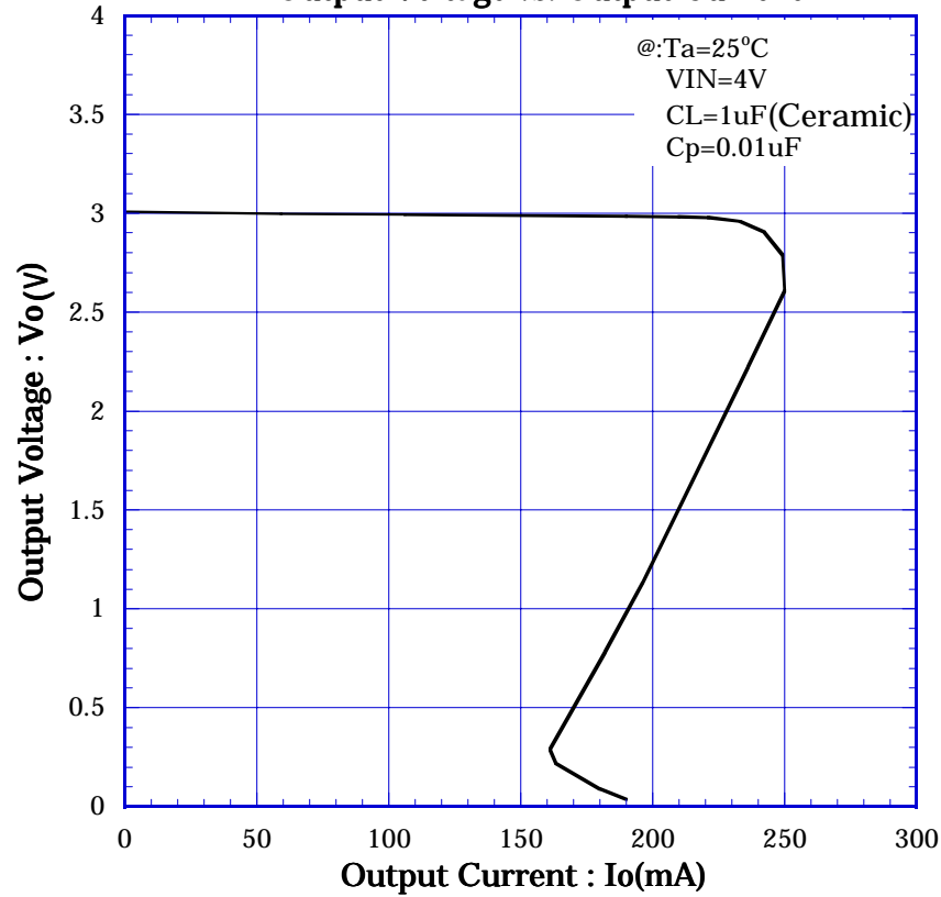
NJM2871/2872_3.0V Output Voltage vs. Output Current
