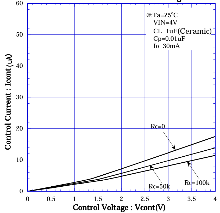
NJM2871/2872_3.0V Control Current vs. Control Voltage
