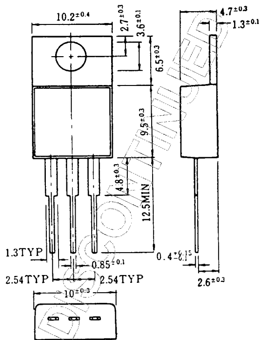
TO-220 Package
