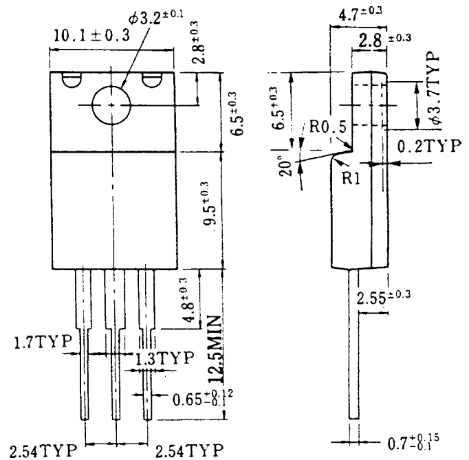
TO-220F Package
